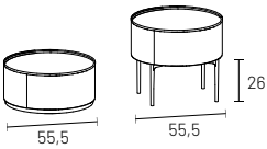
comodino 1 cassetto 1-drawer night stand
