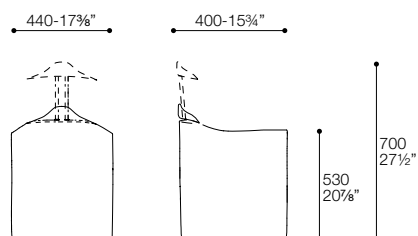
sedia Landscape UP /Landscape Up chair
