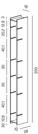
Column 6 slots (sides + back panel)
