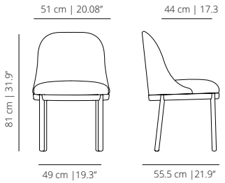
Wooden base chair
