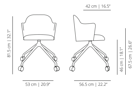
Pyramid casters swivel base chair with arms
