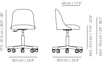
Caster base chair
