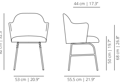
Metal base chair with arms
