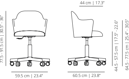
Caster base chair with arms
