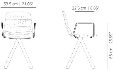
MAB arms
